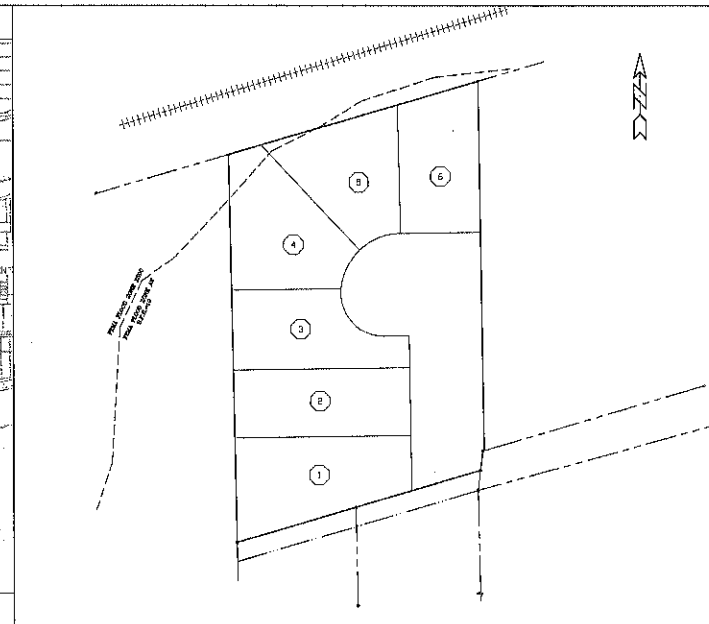
GENERAL LAYOUT
