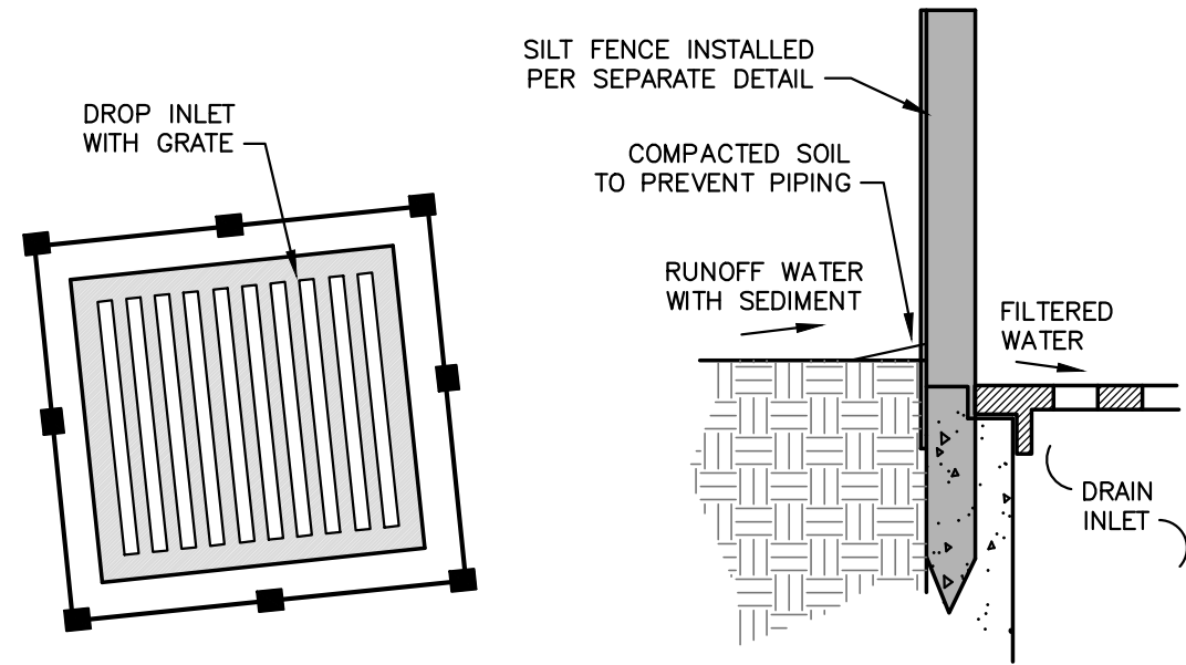
STORM DRAIN INLET PROTECTION
