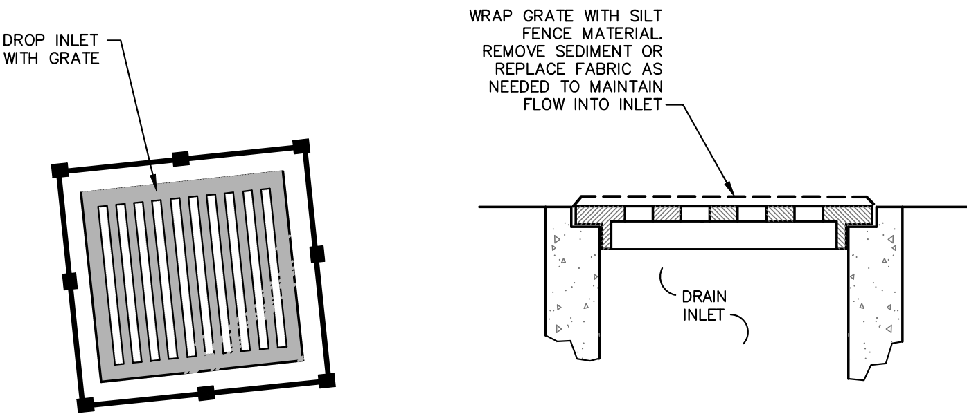
STORM DRAIN INLET PROTECTION
