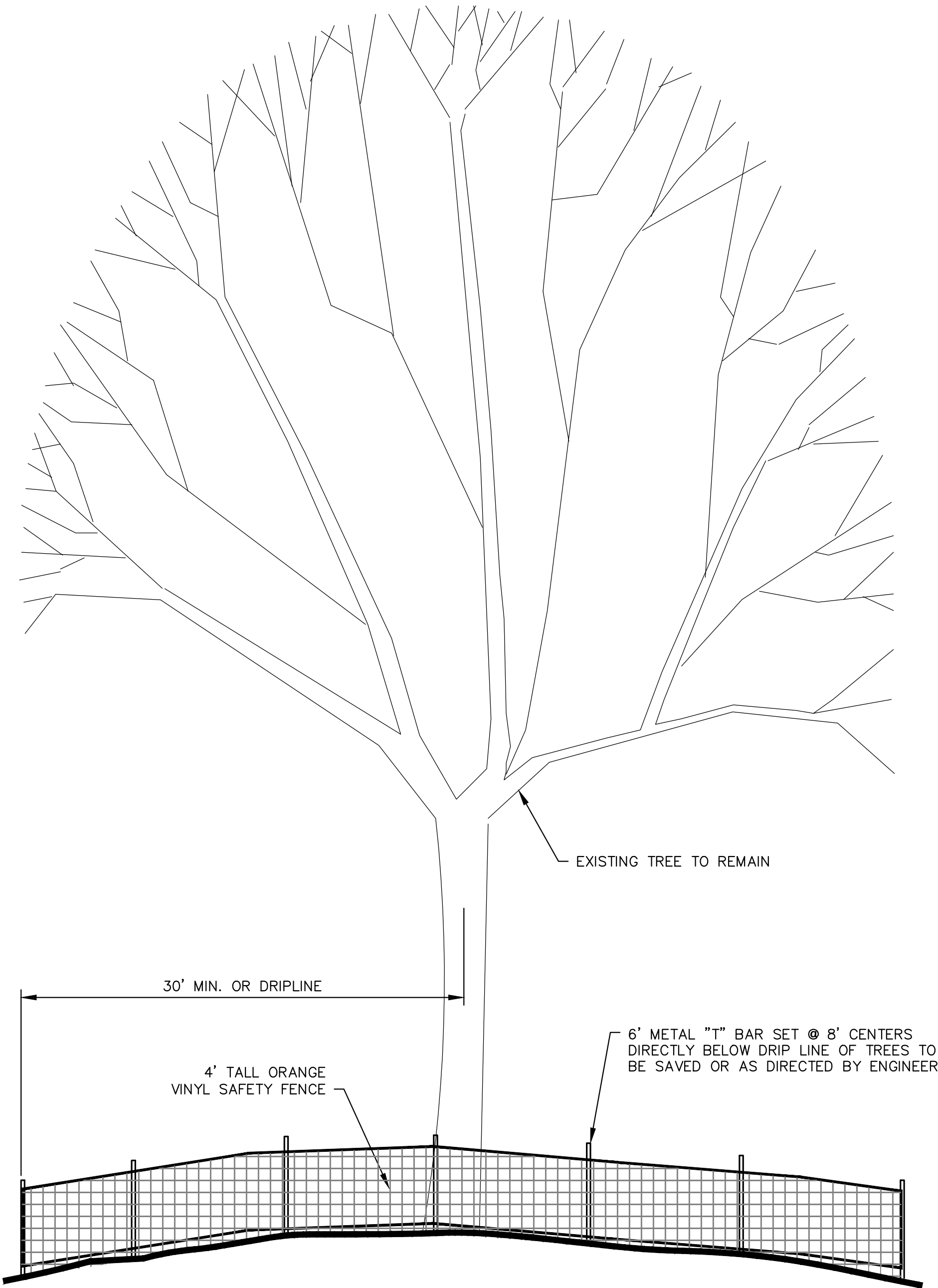
TREE PROTECTION FENCE DETAIL
