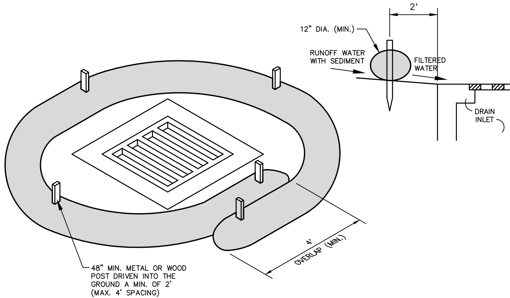
STRAW WATTLE INLET PROTECTION
